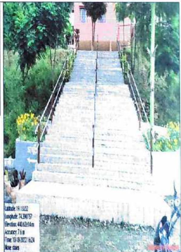
Construction of a sloping staircase in front of the main building
