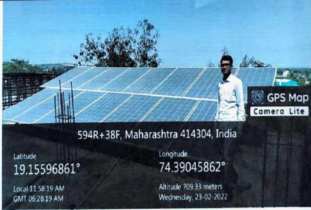
Solar System installed top of Ladies hostel Photo
